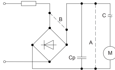
Series circuit
